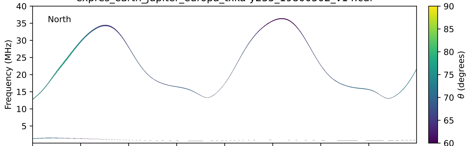
expres_earth_jupiter_europa_txka-y235_19800502_v14.cdf
