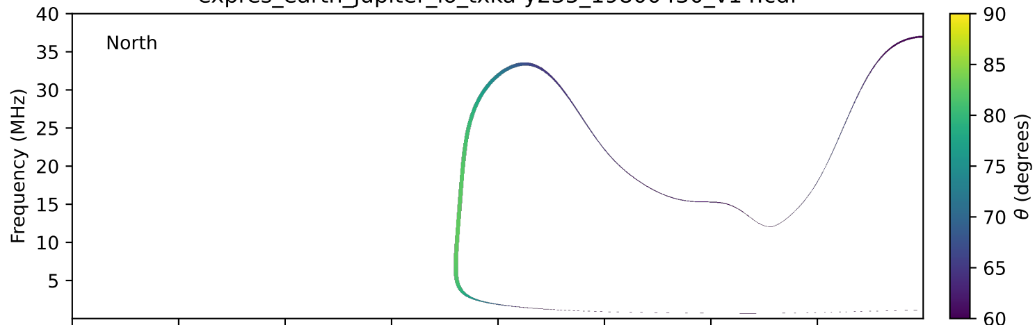
expres_earth_jupiter_io_txka-y235_19800430_v14.cdf
