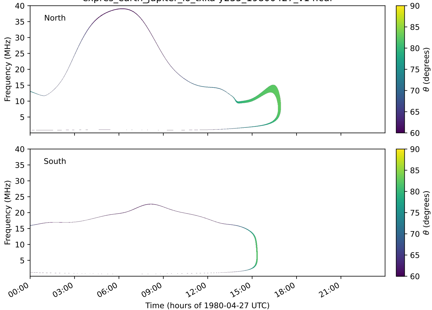
expres_earth_jupiter_io_txka-y235_19800427_v14.cdf
