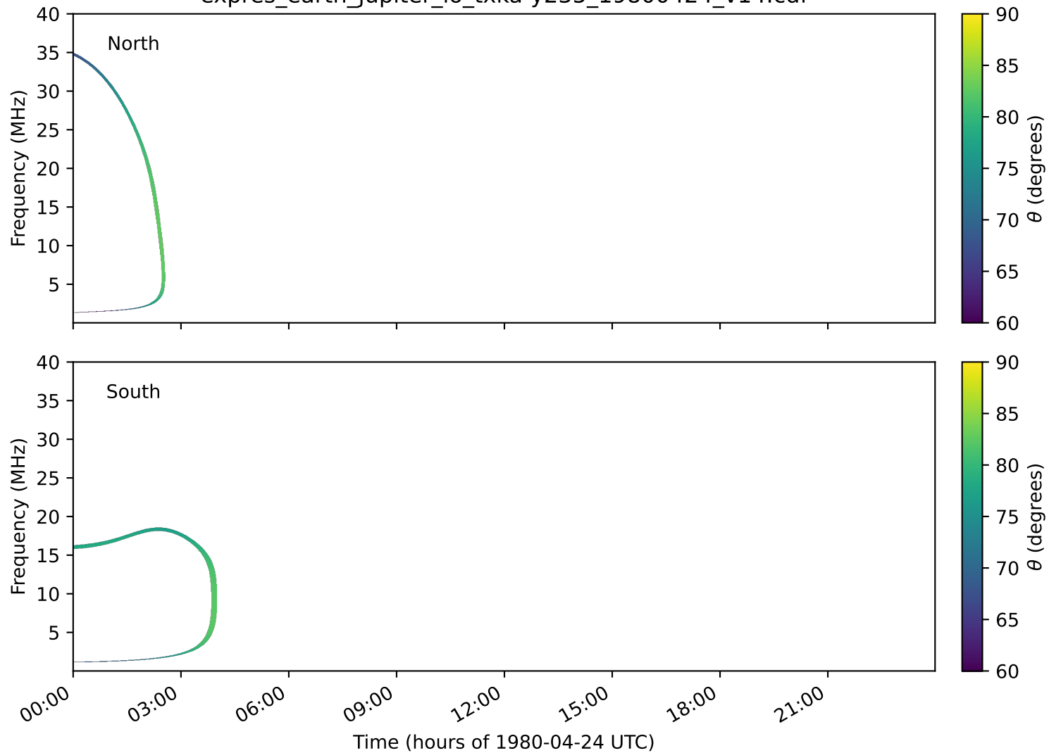
expres_earth_jupiter_io_txka-y235_19800424_v14.cdf
