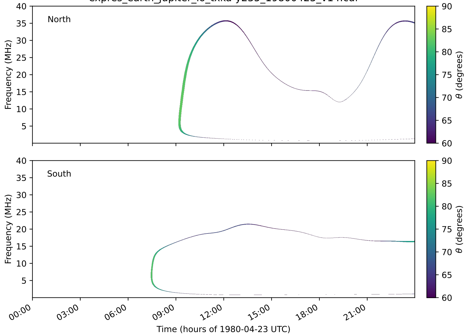
expres_earth_jupiter_io_txka-y235_19800423_v14.cdf
