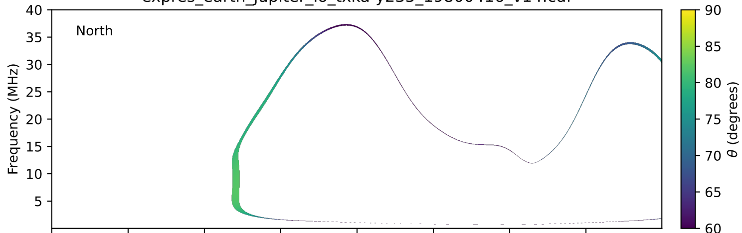
expres_earth_jupiter_io_txka-y235_19800416_v14.cdf
