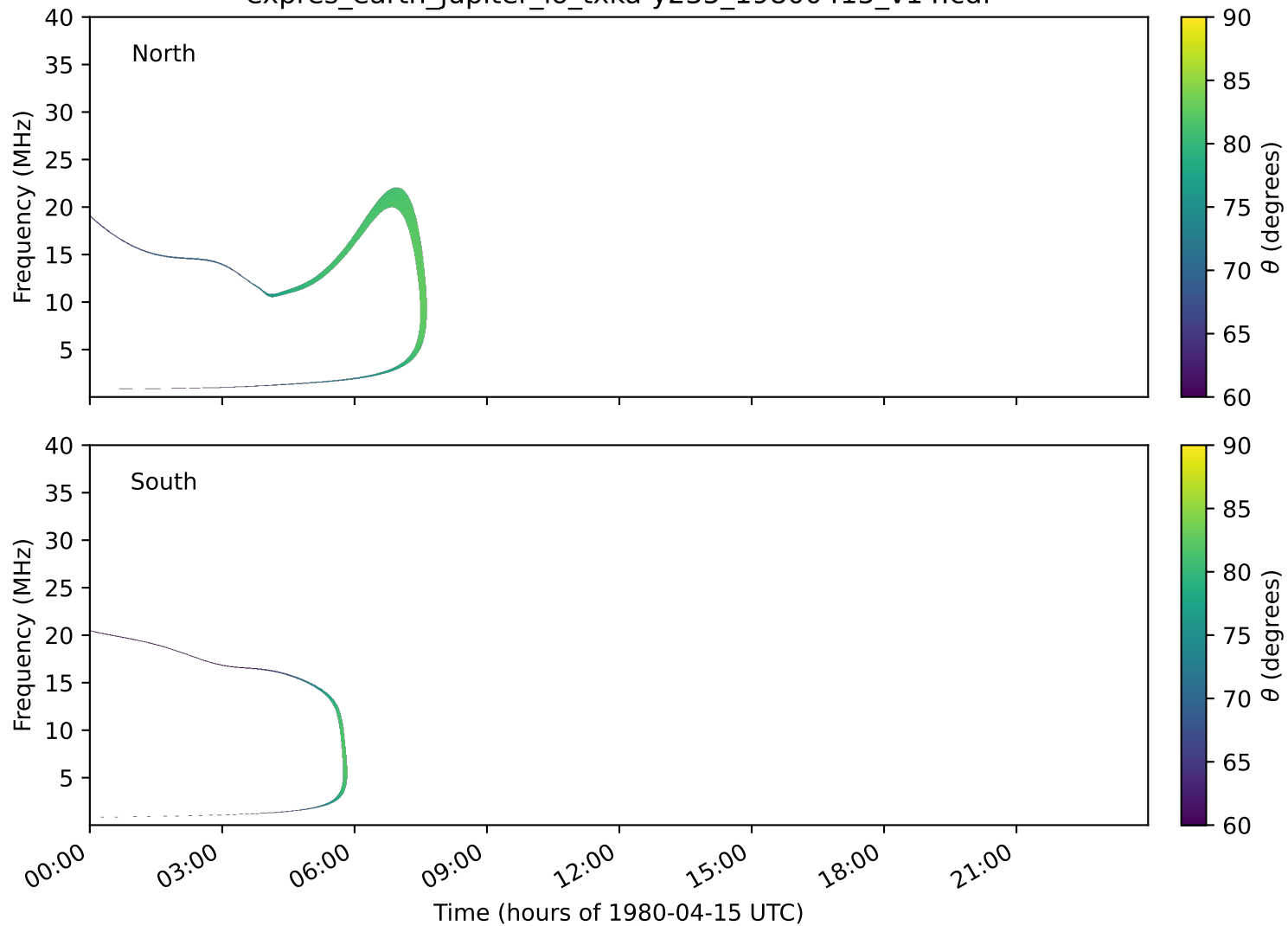
expres_earth_jupiter_io_txka-y235_19800415_v14.cdf
