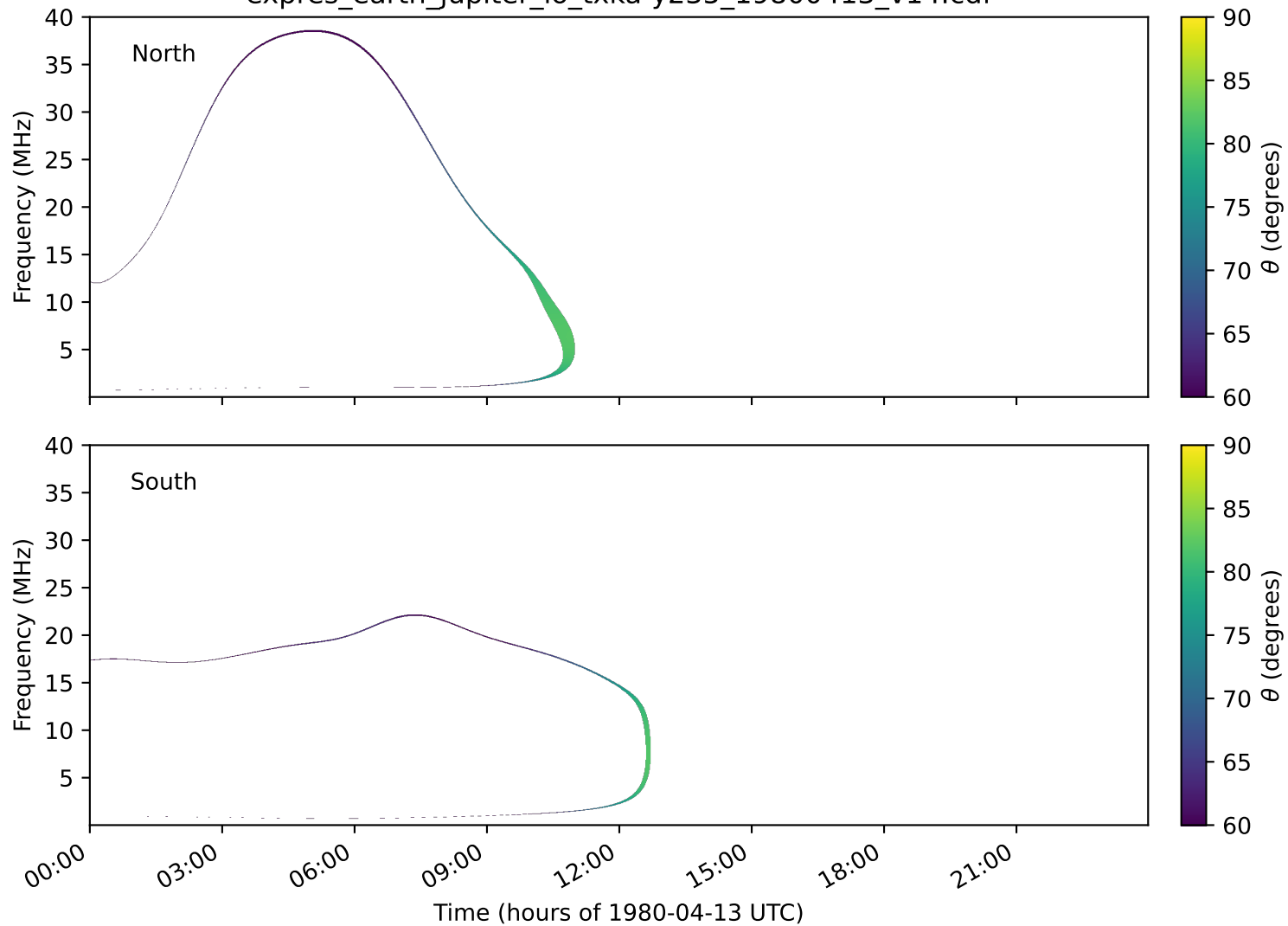
expres_earth_jupiter_io_txka-y235_19800413_v14.cdf
