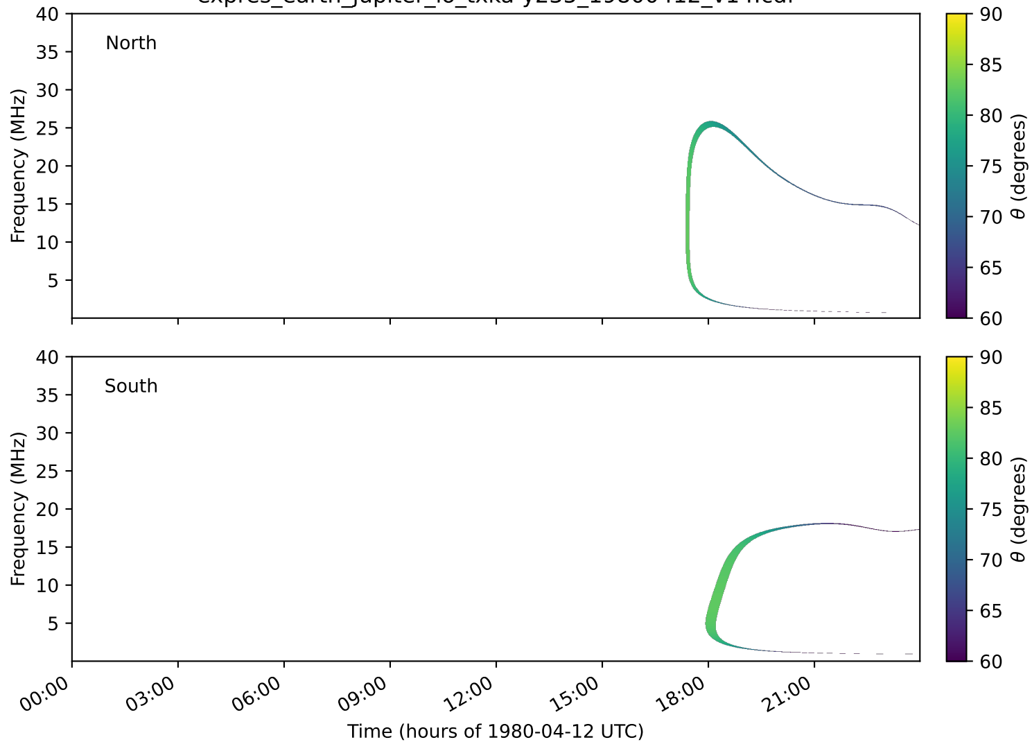
expres_earth_jupiter_io_txka-y235_19800412_v14.cdf
