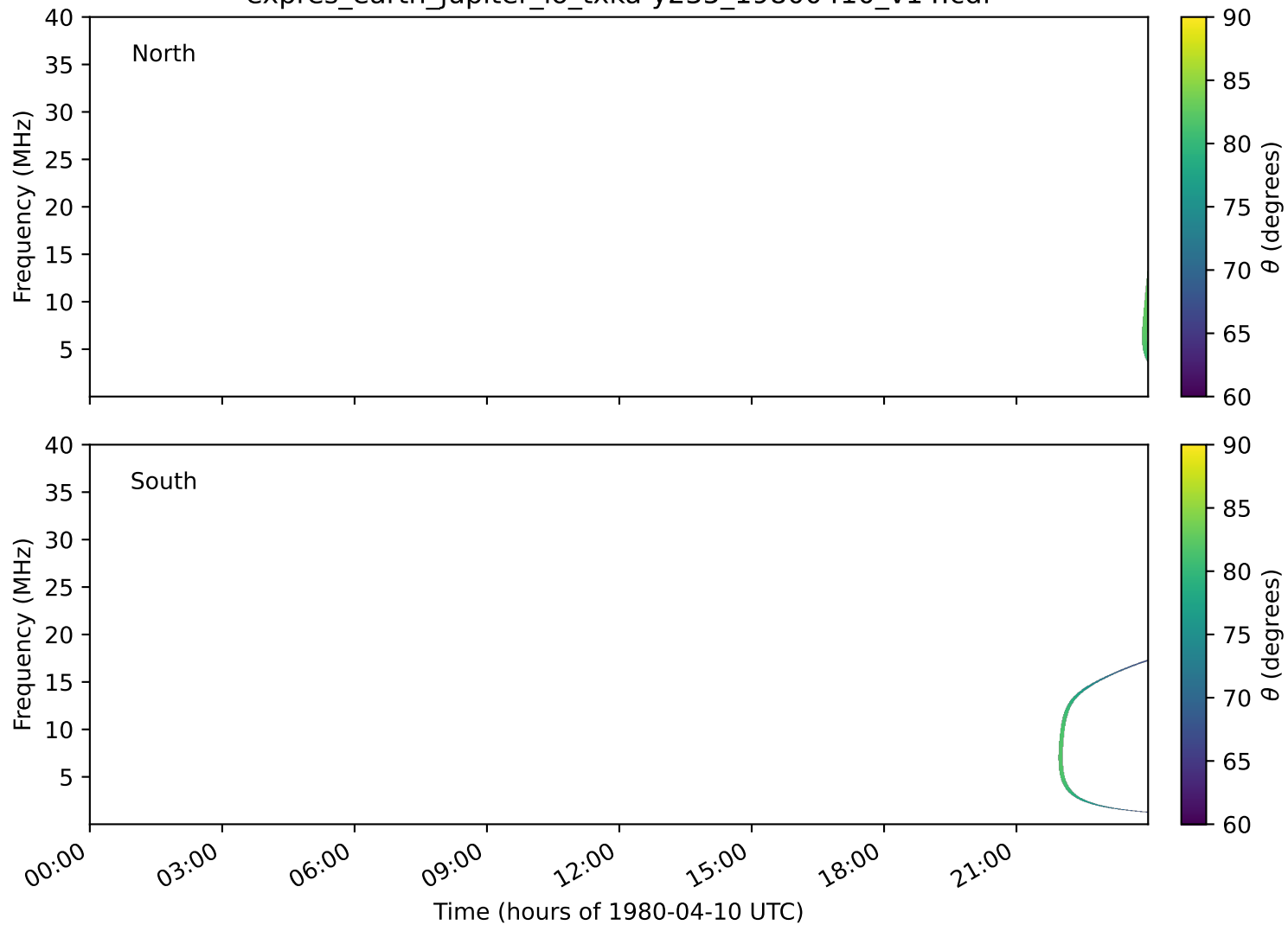
expres_earth_jupiter_io_txka-y235_19800410_v14.cdf
