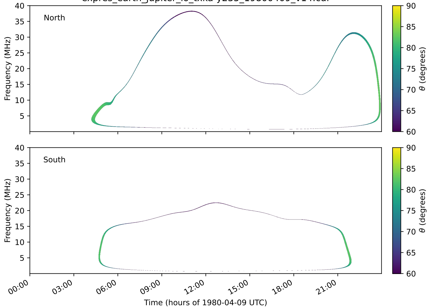
expres_earth_jupiter_io_txka-y235_19800409_v14.cdf
