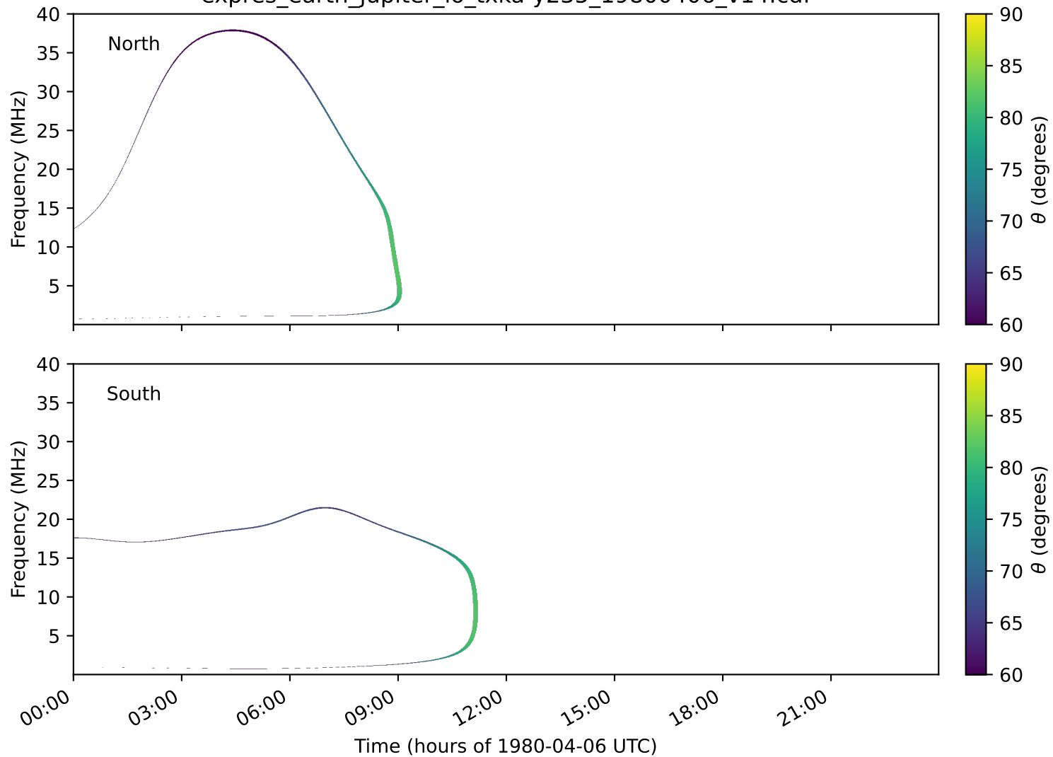
expres_earth_jupiter_io_txka-y235_19800406_v14.cdf
