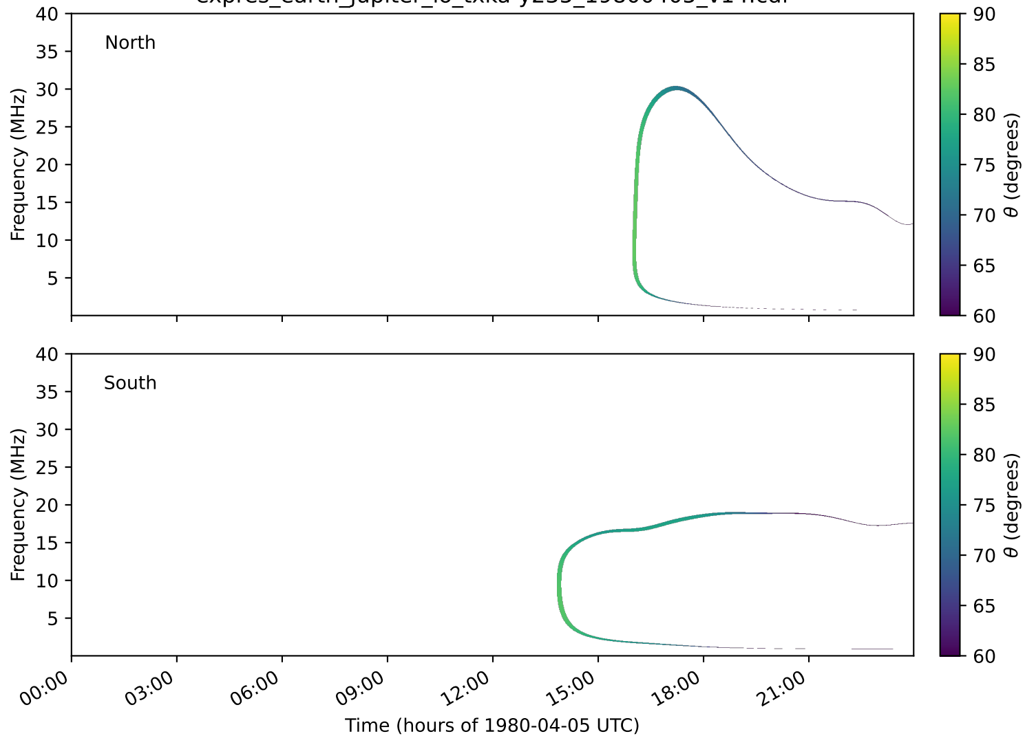
expres_earth_jupiter_io_txka-y235_19800405_v14.cdf
