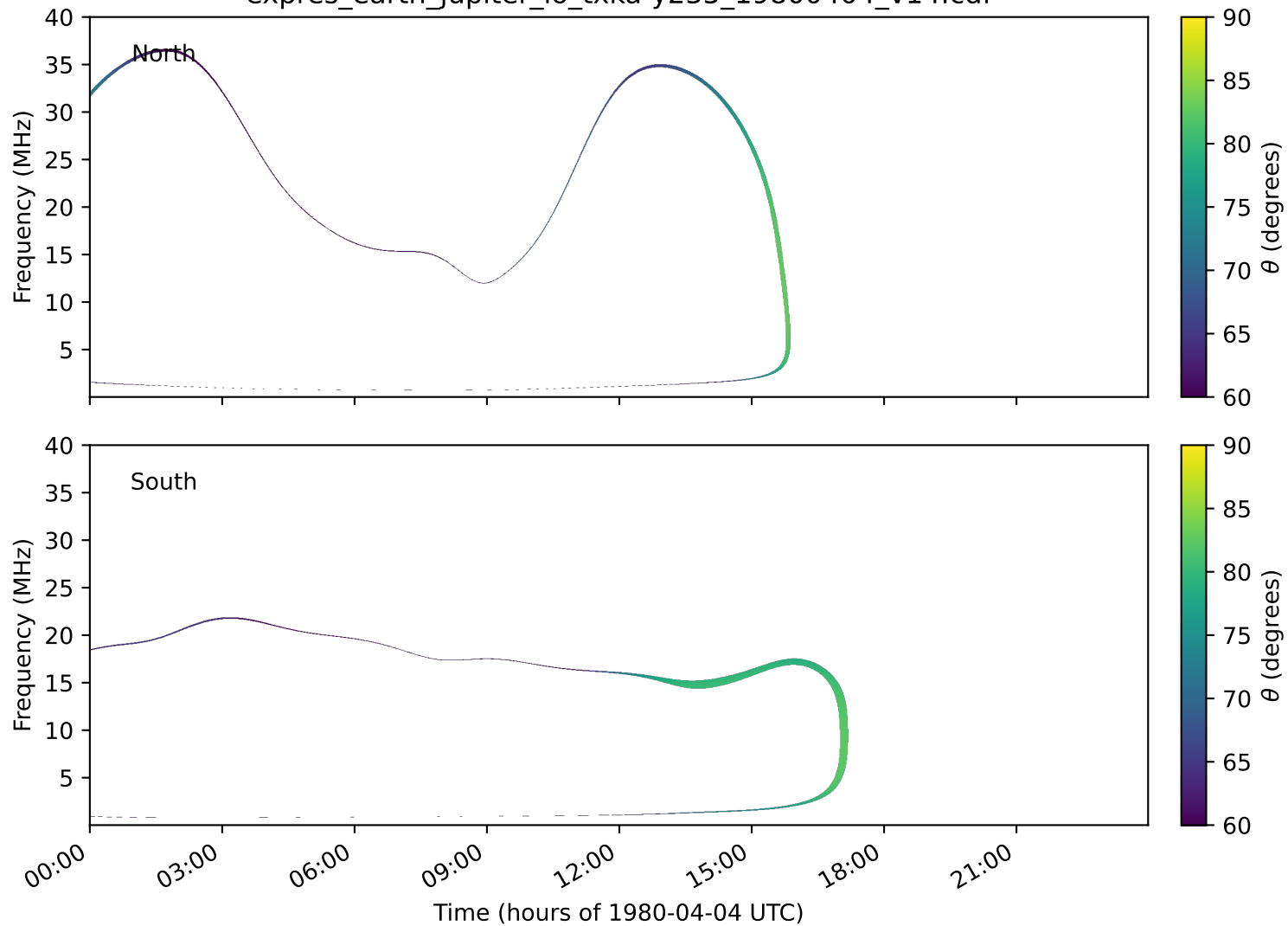
expres_earth_jupiter_io_txka-y235_19800404_v14.cdf
