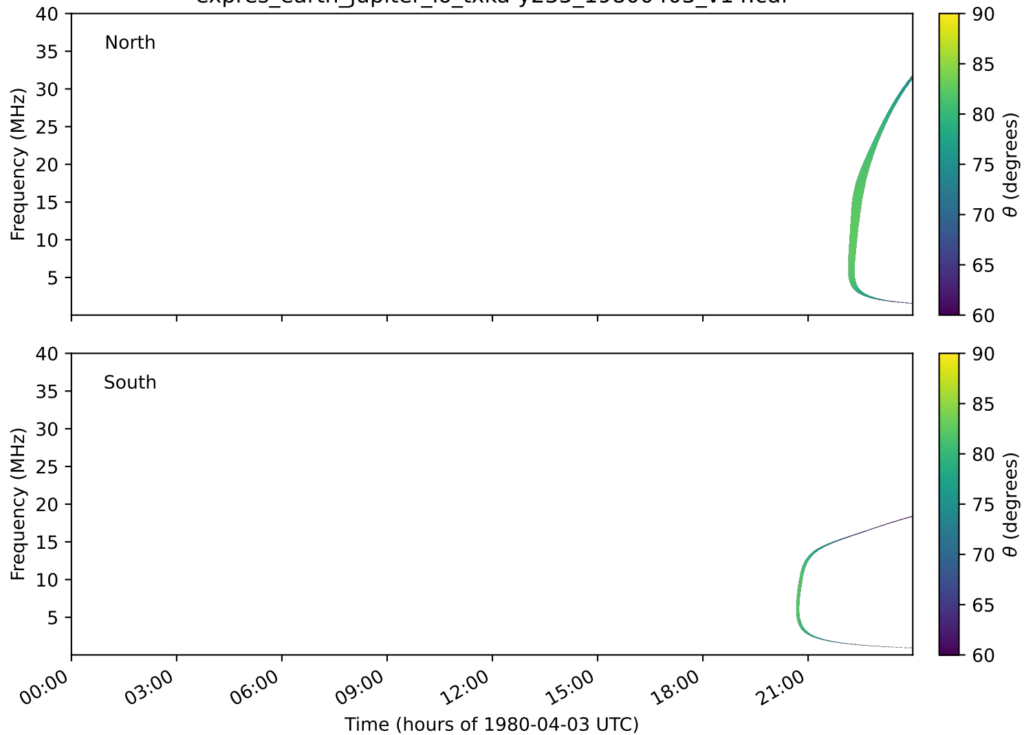
expres_earth_jupiter_io_txka-y235_19800403_v14.cdf
