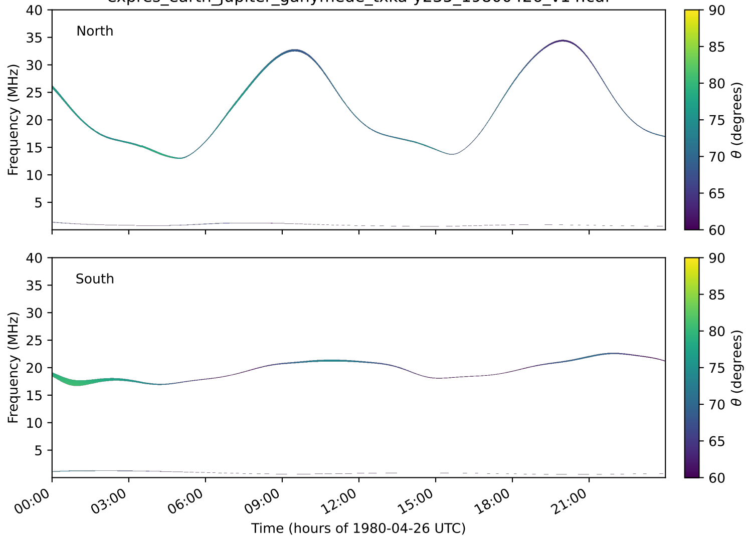
expres_earth_jupiter_ganymede_txka-y235_19800426_v14.cdf
