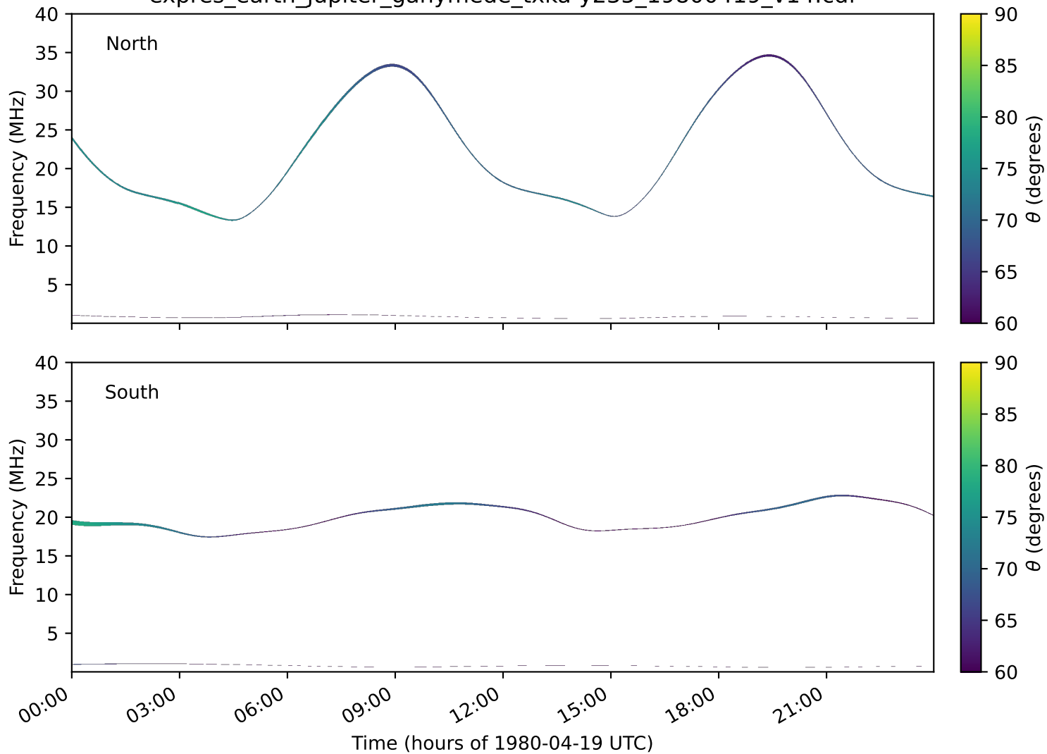
expres_earth_jupiter_ganymede_txka-y235_19800419_v14.cdf
