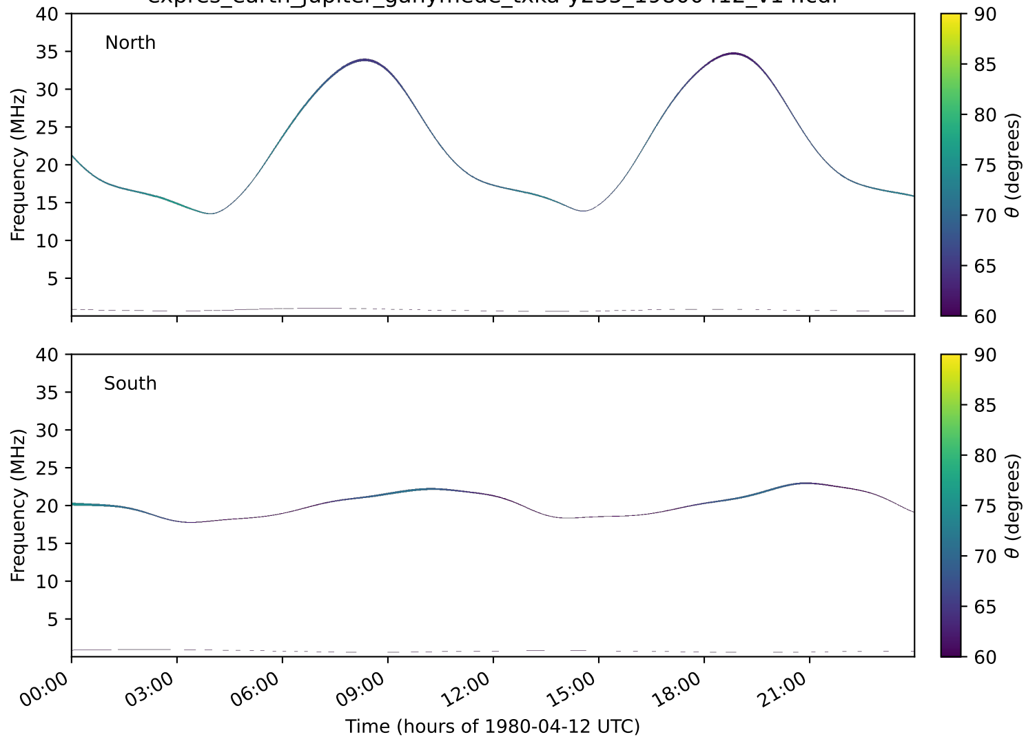
expres_earth_jupiter_ganymede_txka-y235_19800412_v14.cdf
