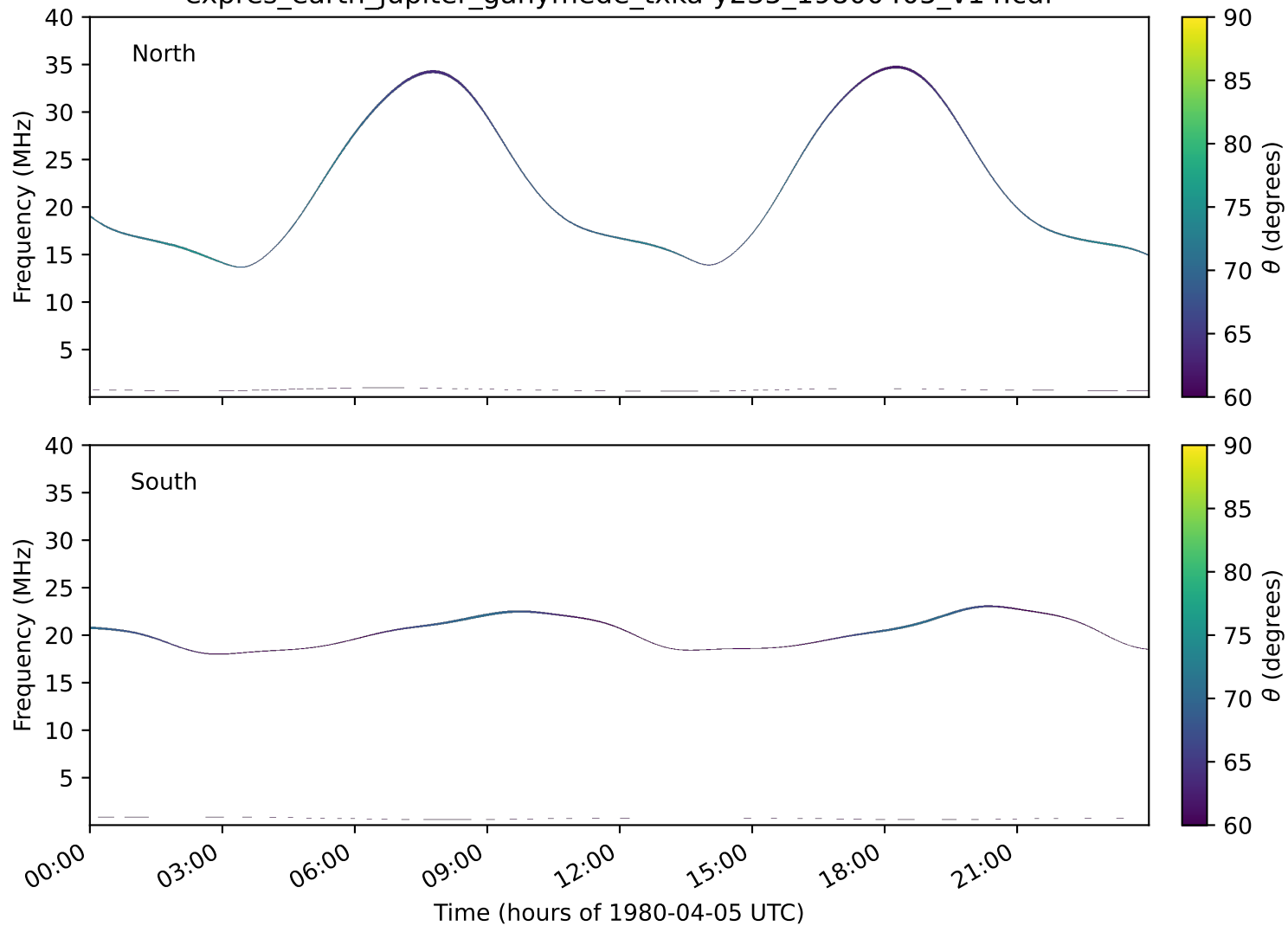
expres_earth_jupiter_ganymede_txka-y235_19800405_v14.cdf
