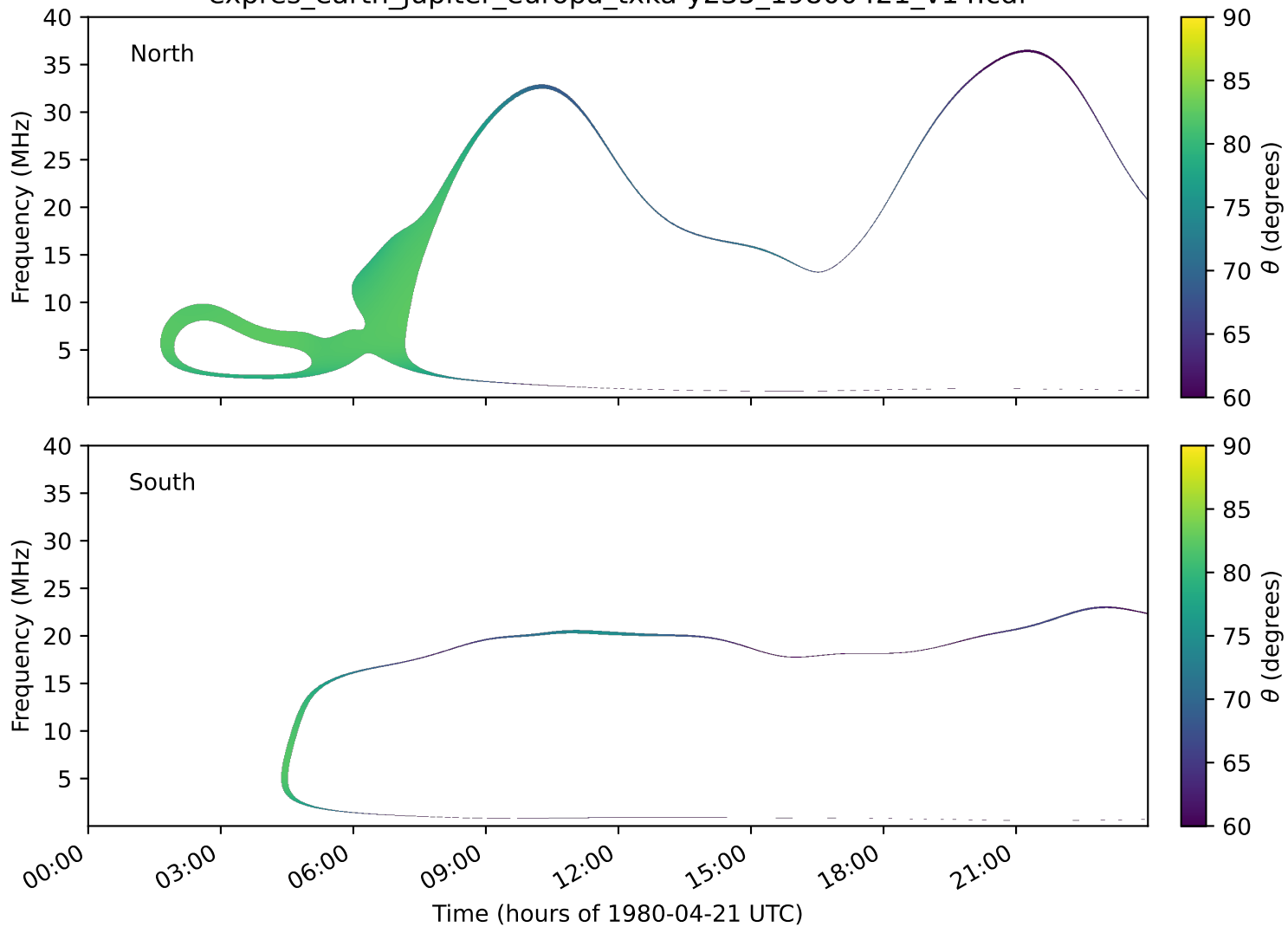
expres_earth_jupiter_europa_txka-y235_19800421_v14.cdf
