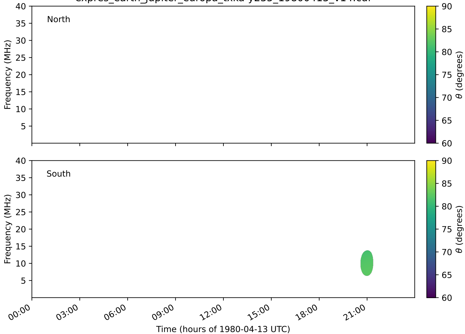
expres_earth_jupiter_europa_txka-y235_19800413_v14.cdf
