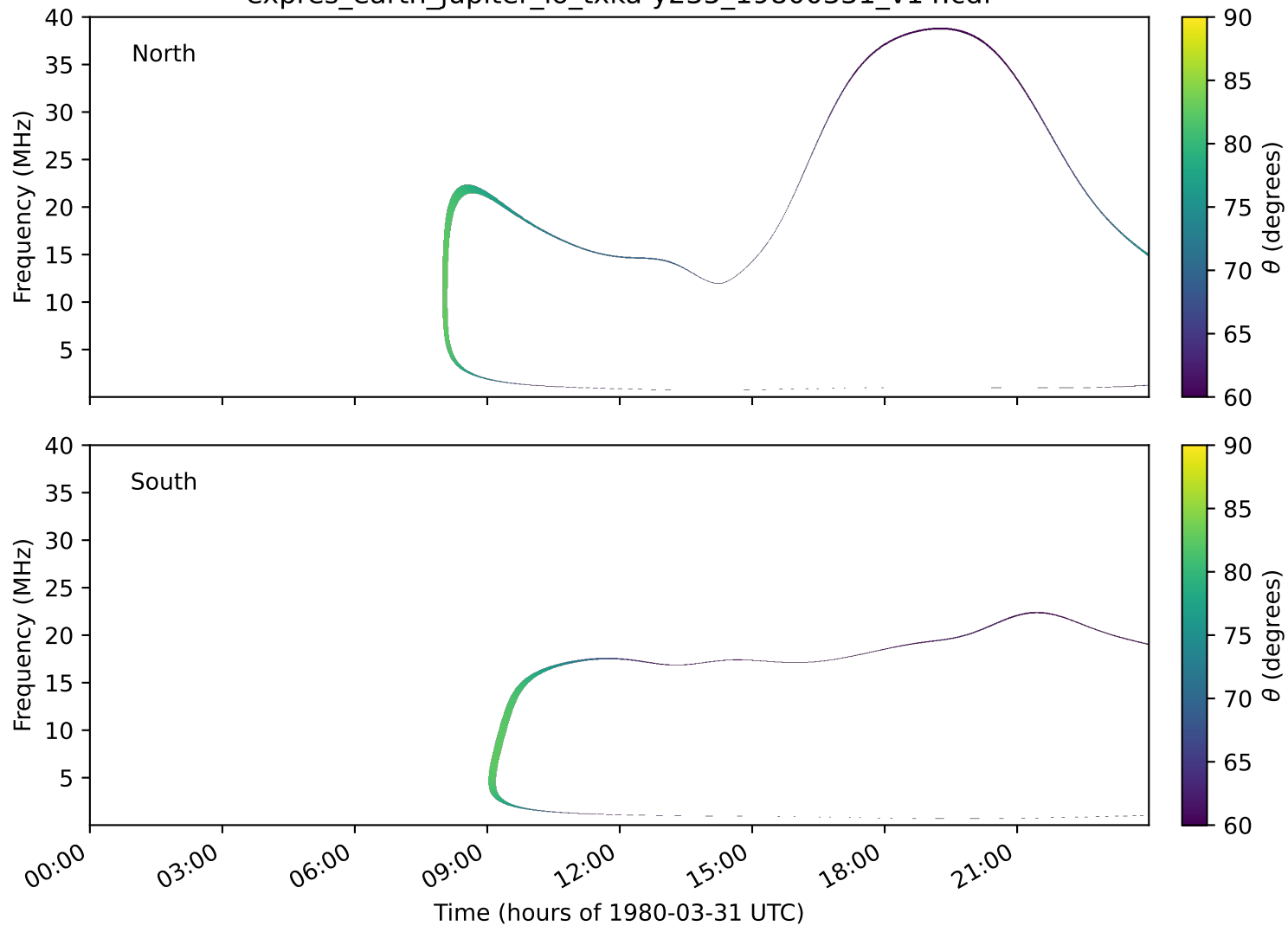
expres_earth_jupiter_io_txka-y235_19800331_v14.cdf
