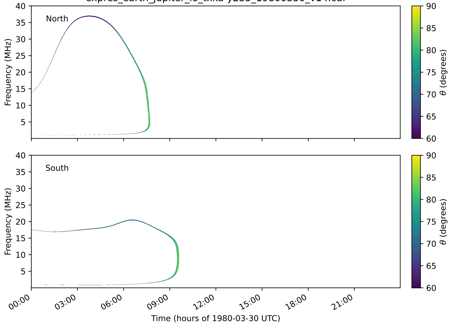
expres_earth_jupiter_io_txka-y235_19800330_v14.cdf
