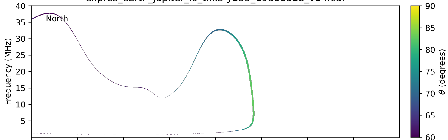
expres_earth_jupiter_io_txka-y235_19800328_v14.cdf
