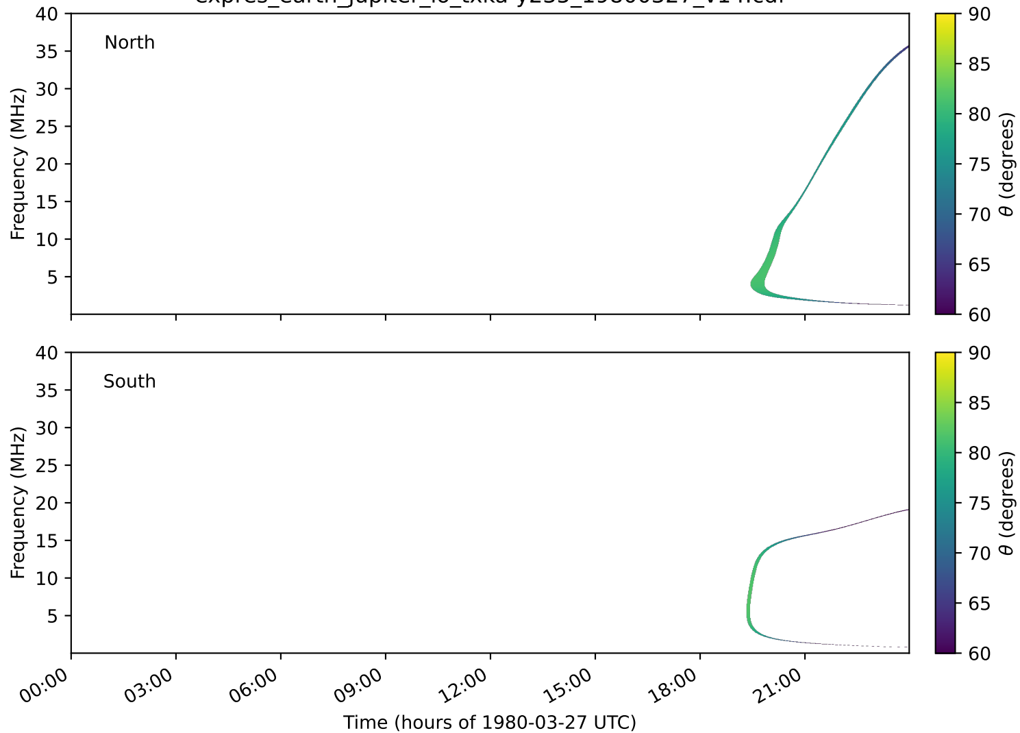
expres_earth_jupiter_io_txka-y235_19800327_v14.cdf
