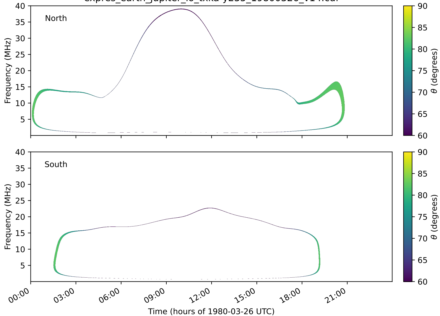
expres_earth_jupiter_io_txka-y235_19800326_v14.cdf
