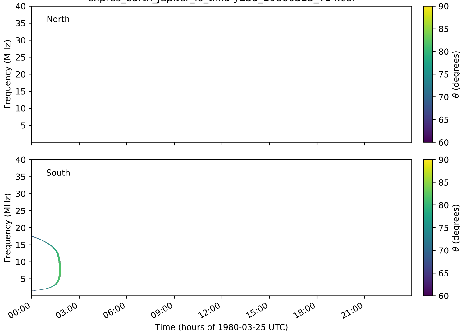
expres_earth_jupiter_io_txka-y235_19800325_v14.cdf
