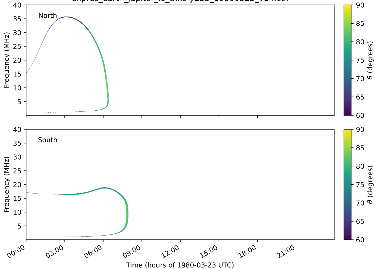
expres_earth_jupiter_io_txka-y235_19800323_v14.cdf
