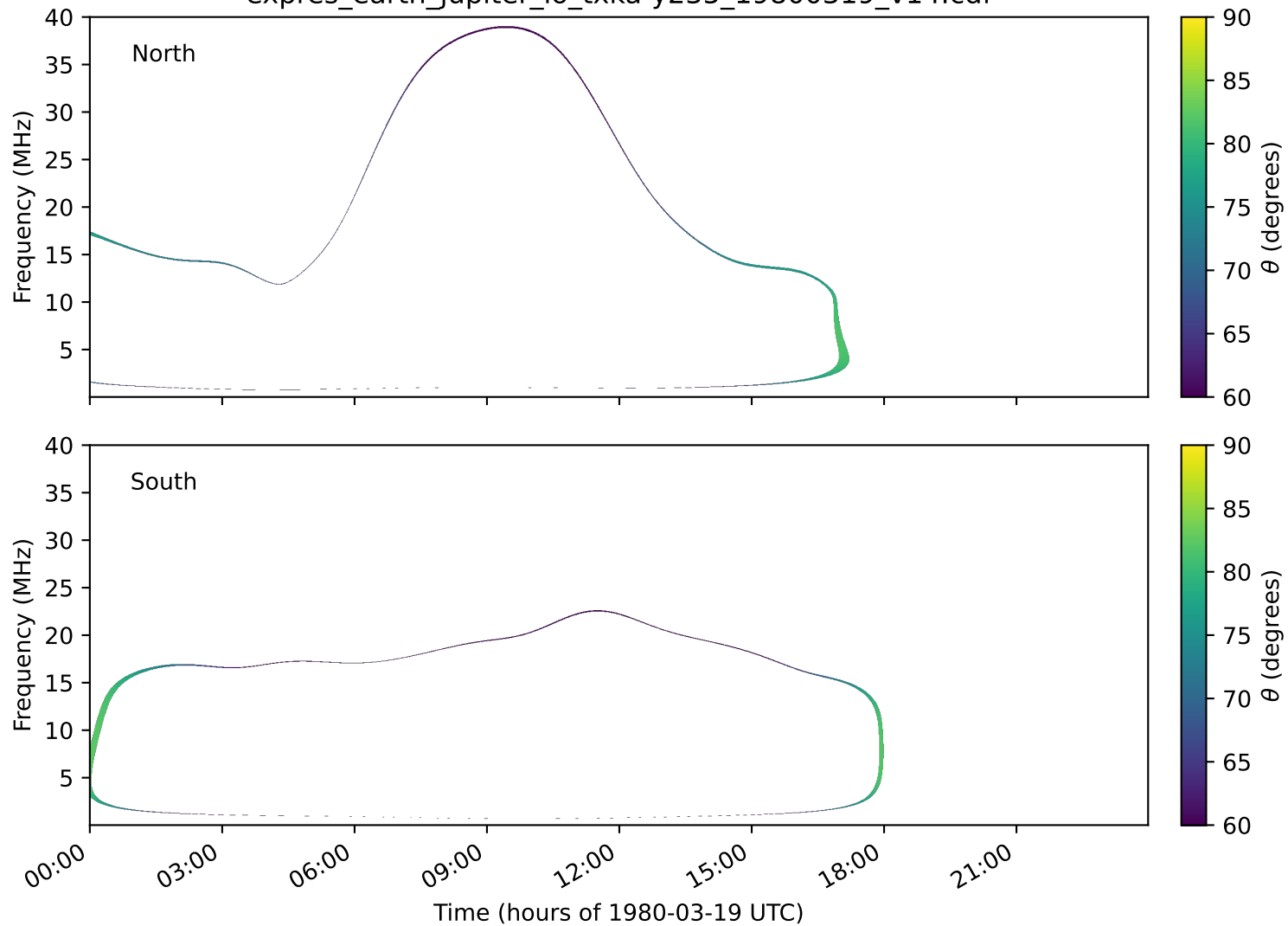
expres_earth_jupiter_io_txka-y235_19800319_v14.cdf
