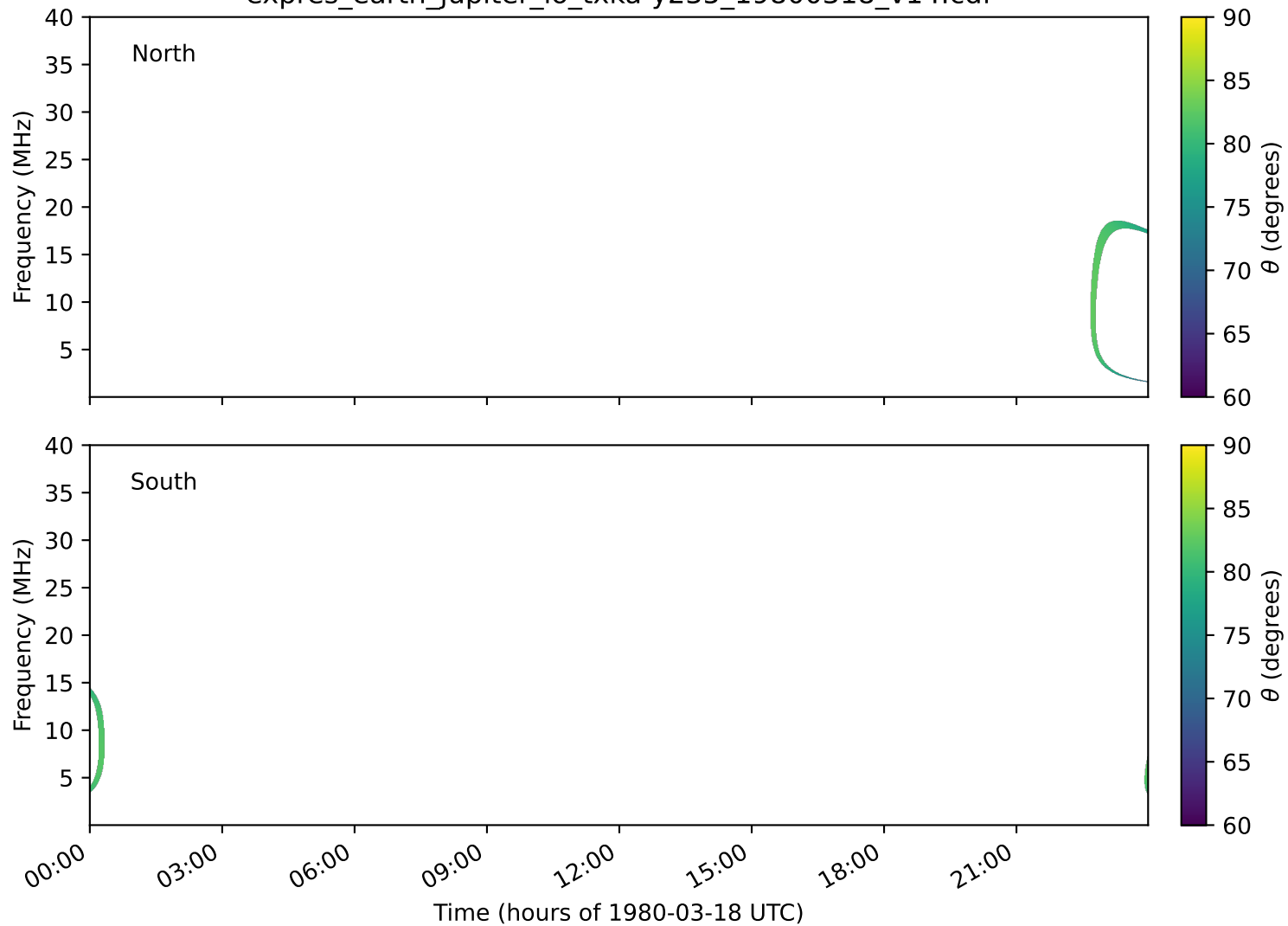
expres_earth_jupiter_io_txka-y235_19800318_v14.cdf
