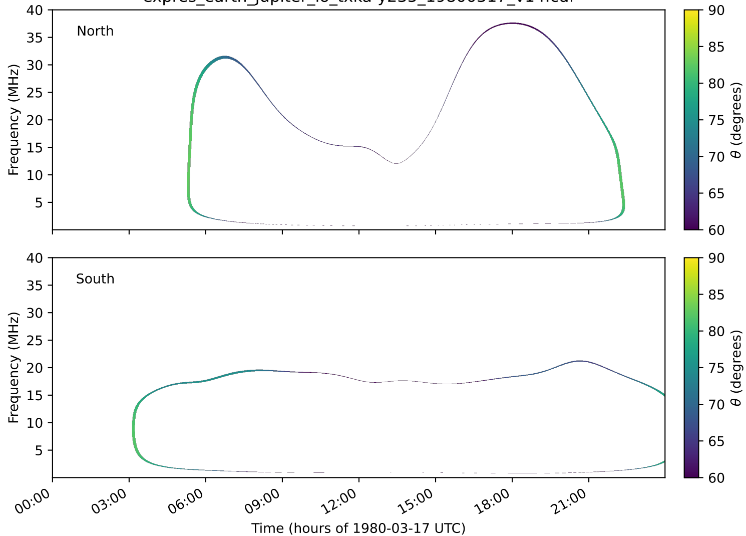
expres_earth_jupiter_io_txka-y235_19800317_v14.cdf
