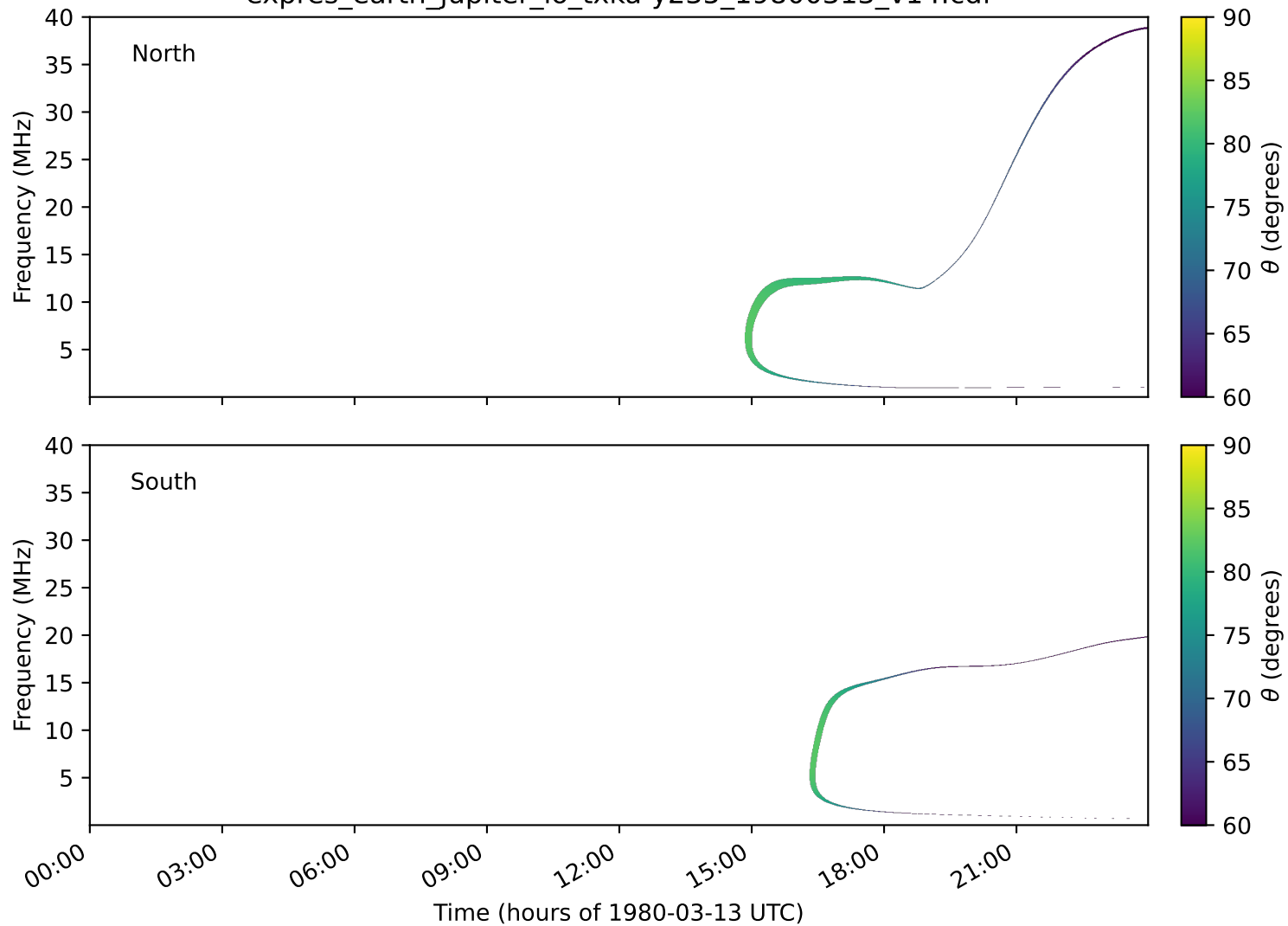
expres_earth_jupiter_io_txka-y235_19800313_v14.cdf
