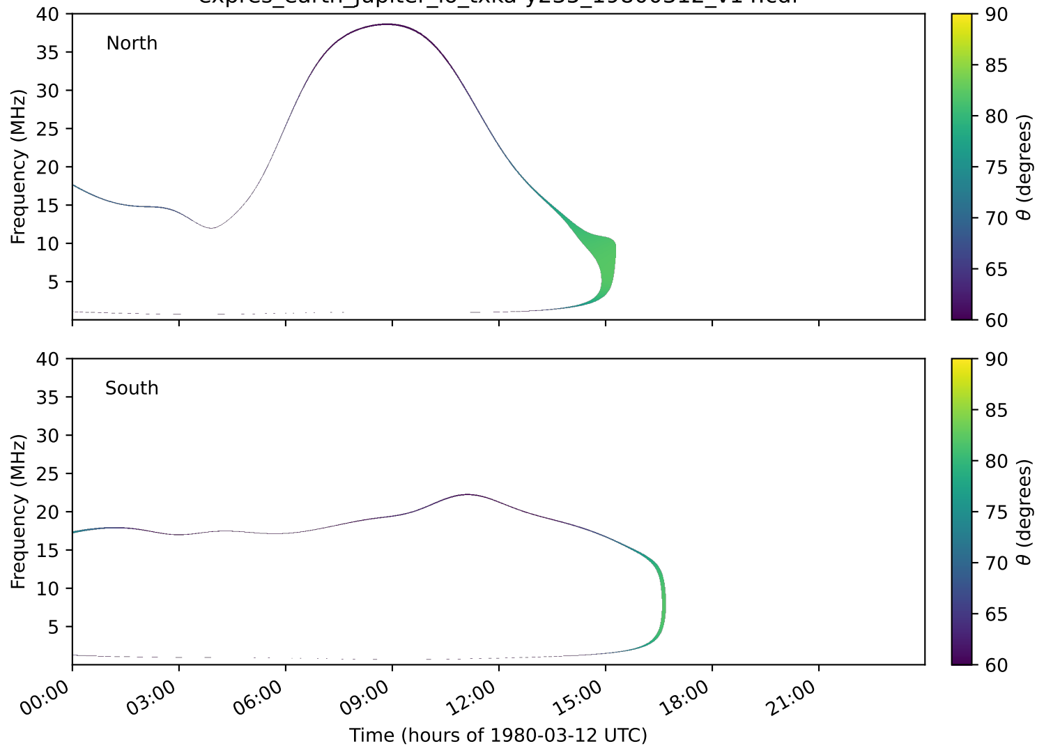
expres_earth_jupiter_io_txka-y235_19800312_v14.cdf
