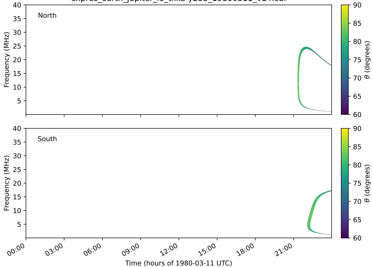
expres_earth_jupiter_io_txka-y235_19800311_v14.cdf
