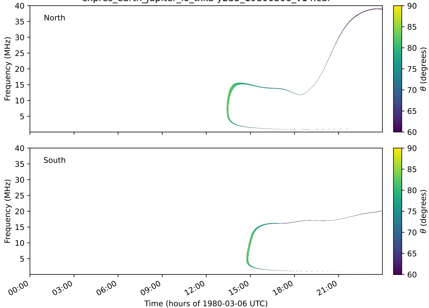
expres_earth_jupiter_io_txka-y235_19800306_v14.cdf
