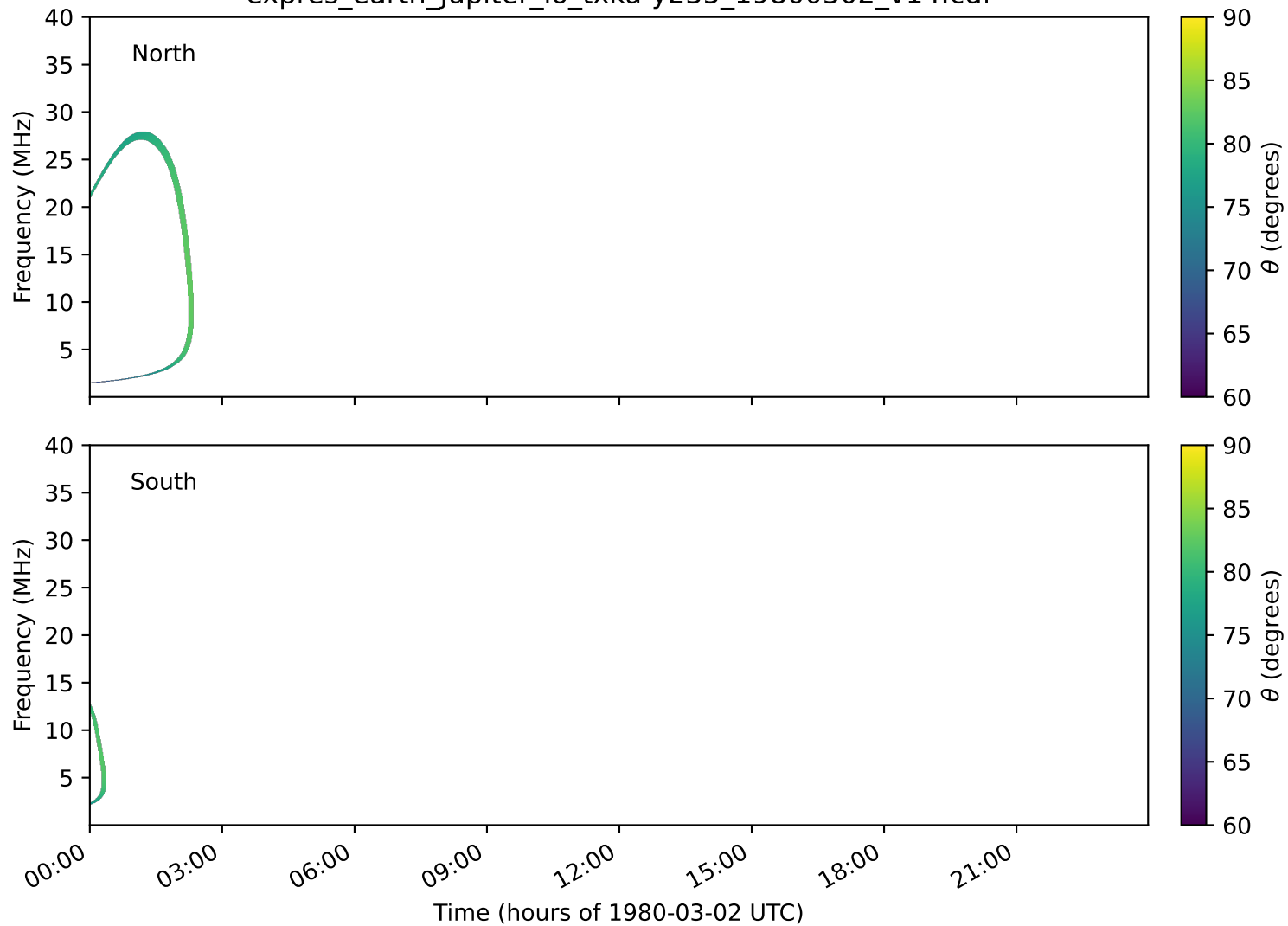
expres_earth_jupiter_io_txka-y235_19800302_v14.cdf
