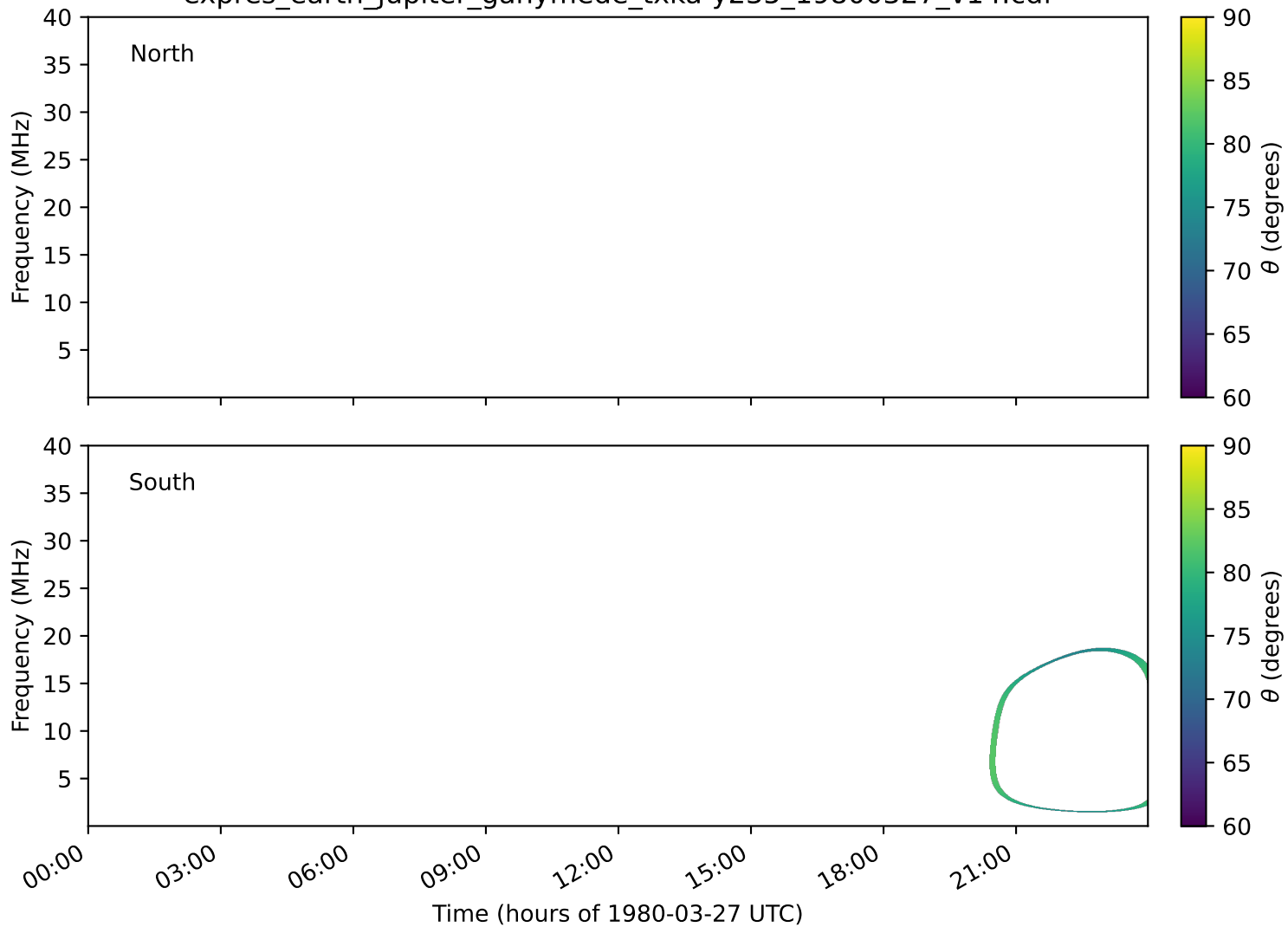
expres_earth_jupiter_ganymede_txka-y235_19800327_v14.cdf
