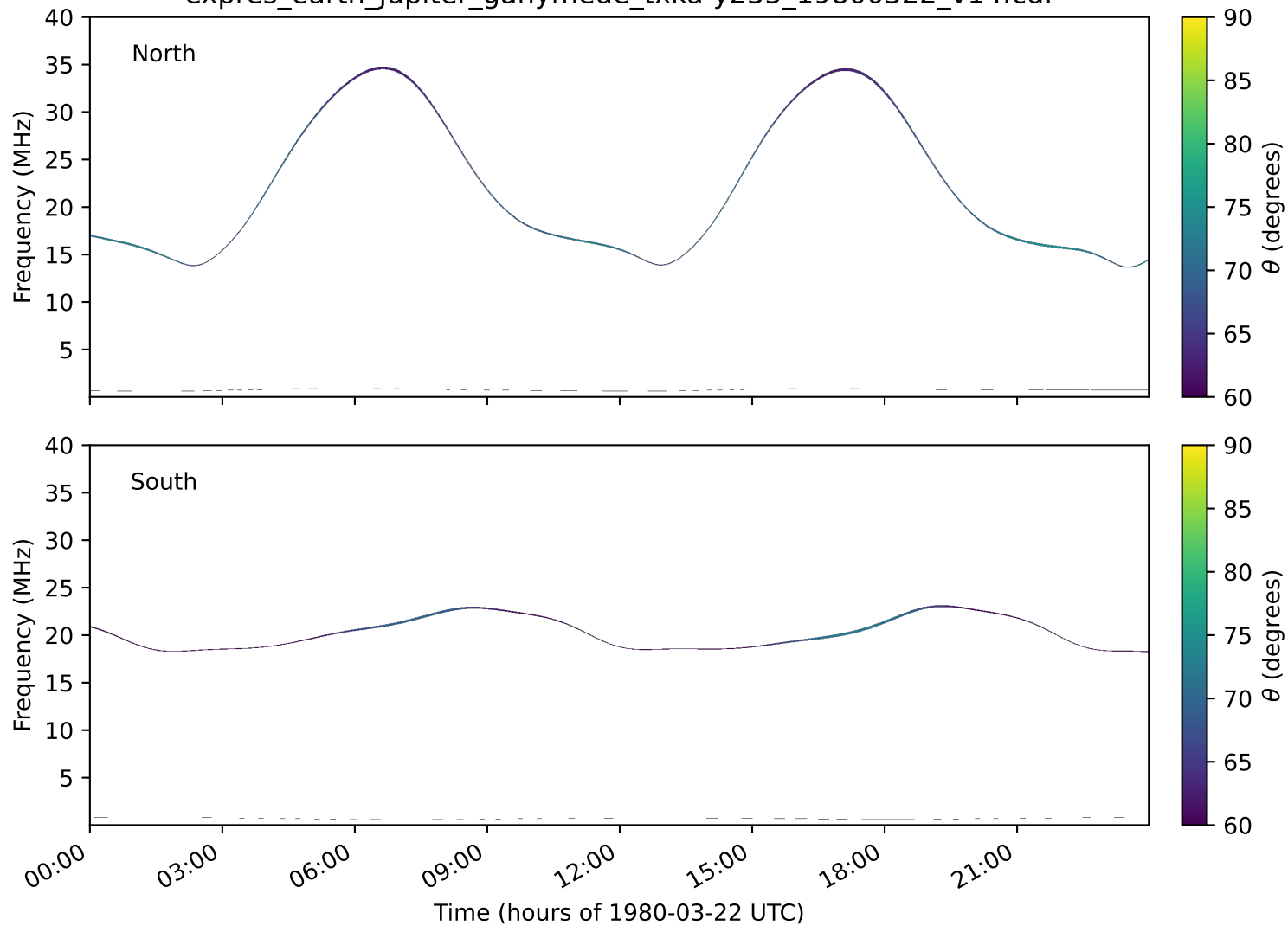
expres_earth_jupiter_ganymede_txka-y235_19800322_v14.cdf
