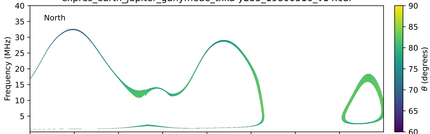
expres_earth_jupiter_ganymede_txka-y235_19800316_v14.cdf
