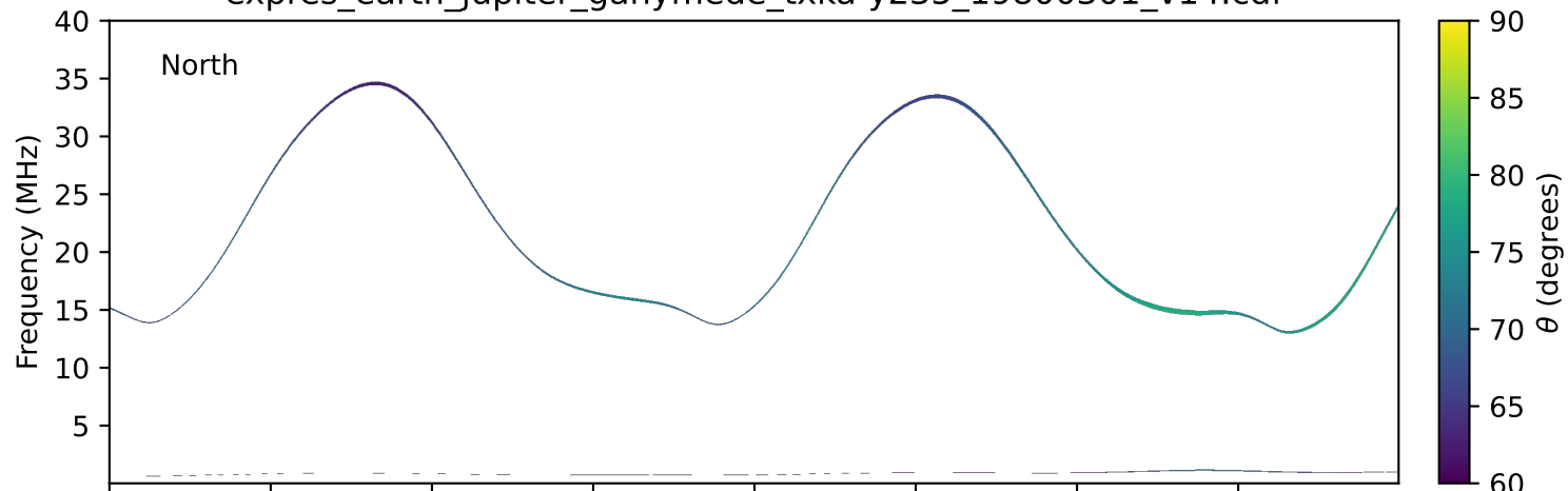
expres_earth_jupiter_ganymede_txka-y235_19800301_v14.cdf
