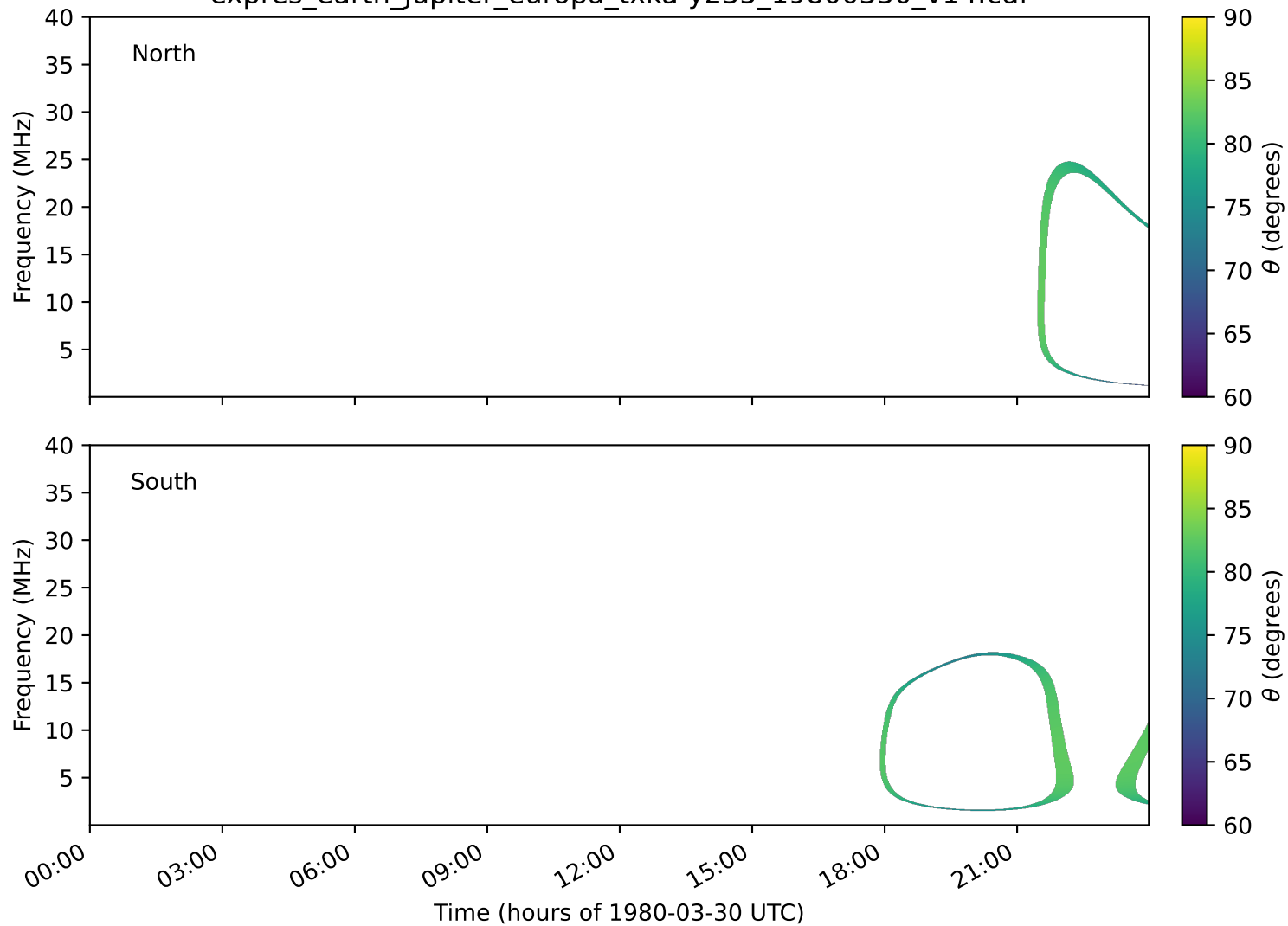
expres_earth_jupiter_europa_txka-y235_19800330_v14.cdf
