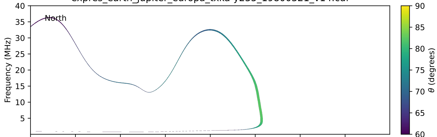
expres_earth_jupiter_europa_txka-y235_19800321_v14.cdf
