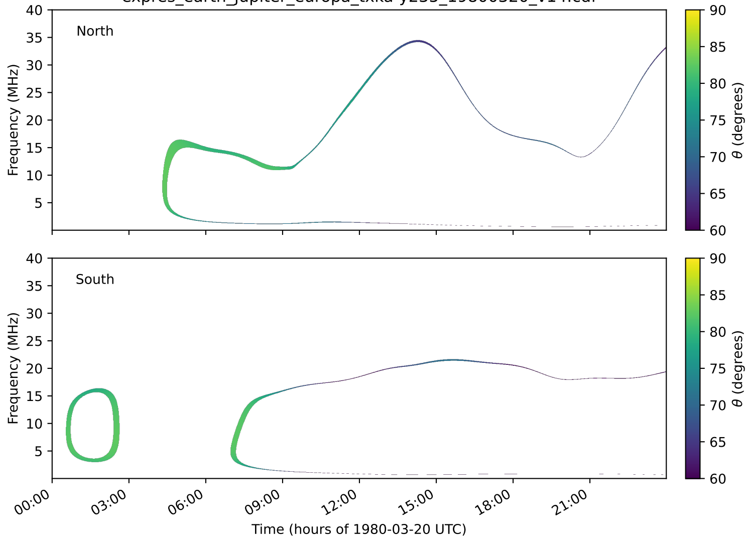
expres_earth_jupiter_europa_txka-y235_19800320_v14.cdf
