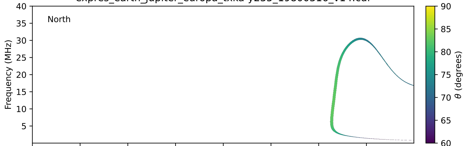
expres_earth_jupiter_europa_txka-y235_19800316_v14.cdf
