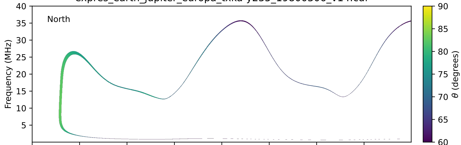
expres_earth_jupiter_europa_txka-y235_19800306_v14.cdf
