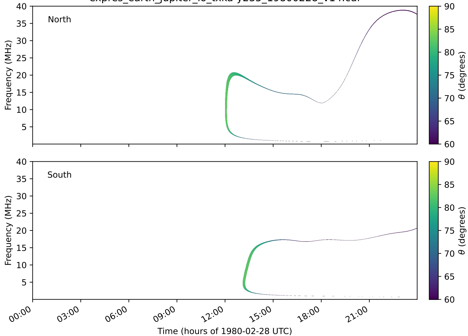
expres_earth_jupiter_io_txka-y235_19800228_v14.cdf
