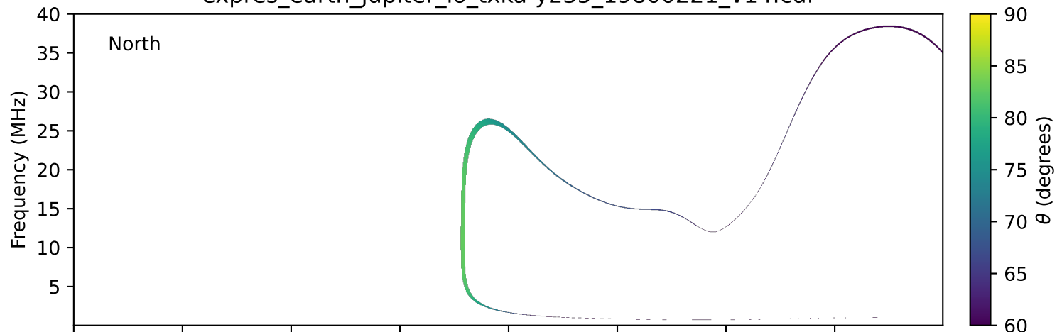
expres_earth_jupiter_io_txka-y235_19800221_v14.cdf
