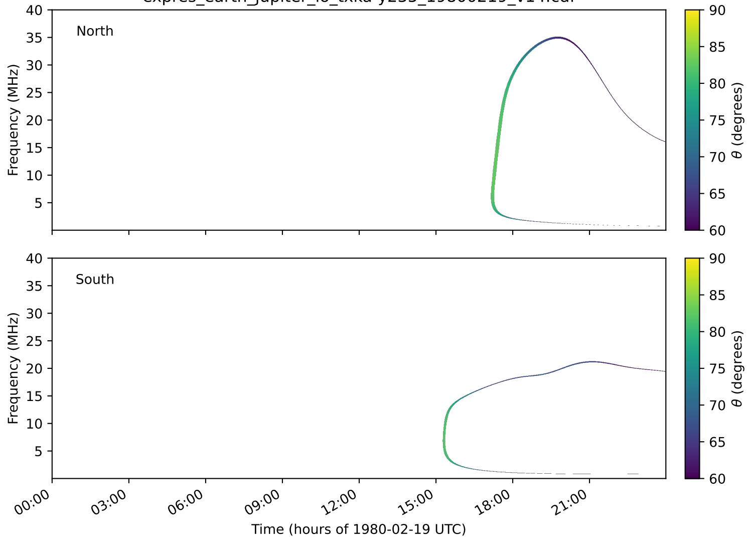
expres_earth_jupiter_io_txka-y235_19800219_v14.cdf
