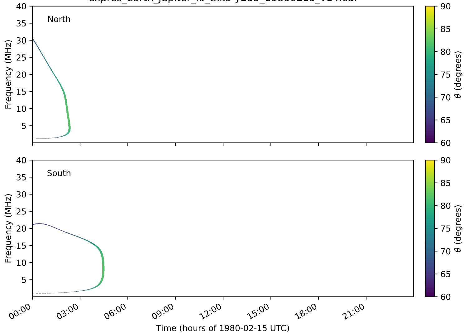
expres_earth_jupiter_io_txka-y235_19800215_v14.cdf
