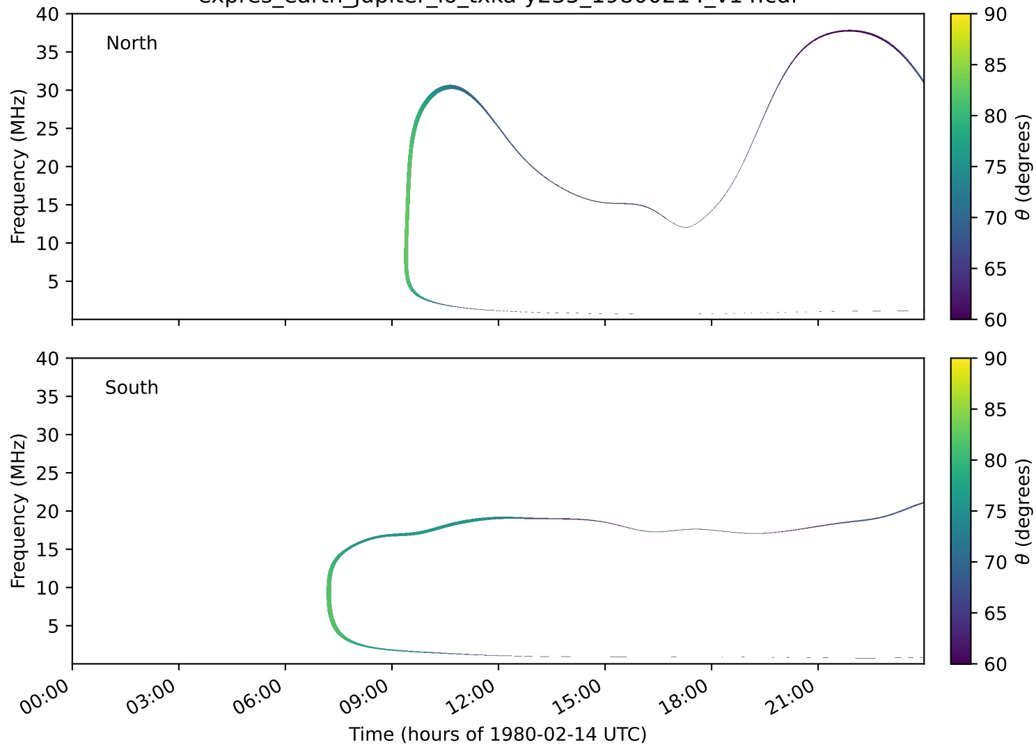
expres_earth_jupiter_io_txka-y235_19800214_v14.cdf
